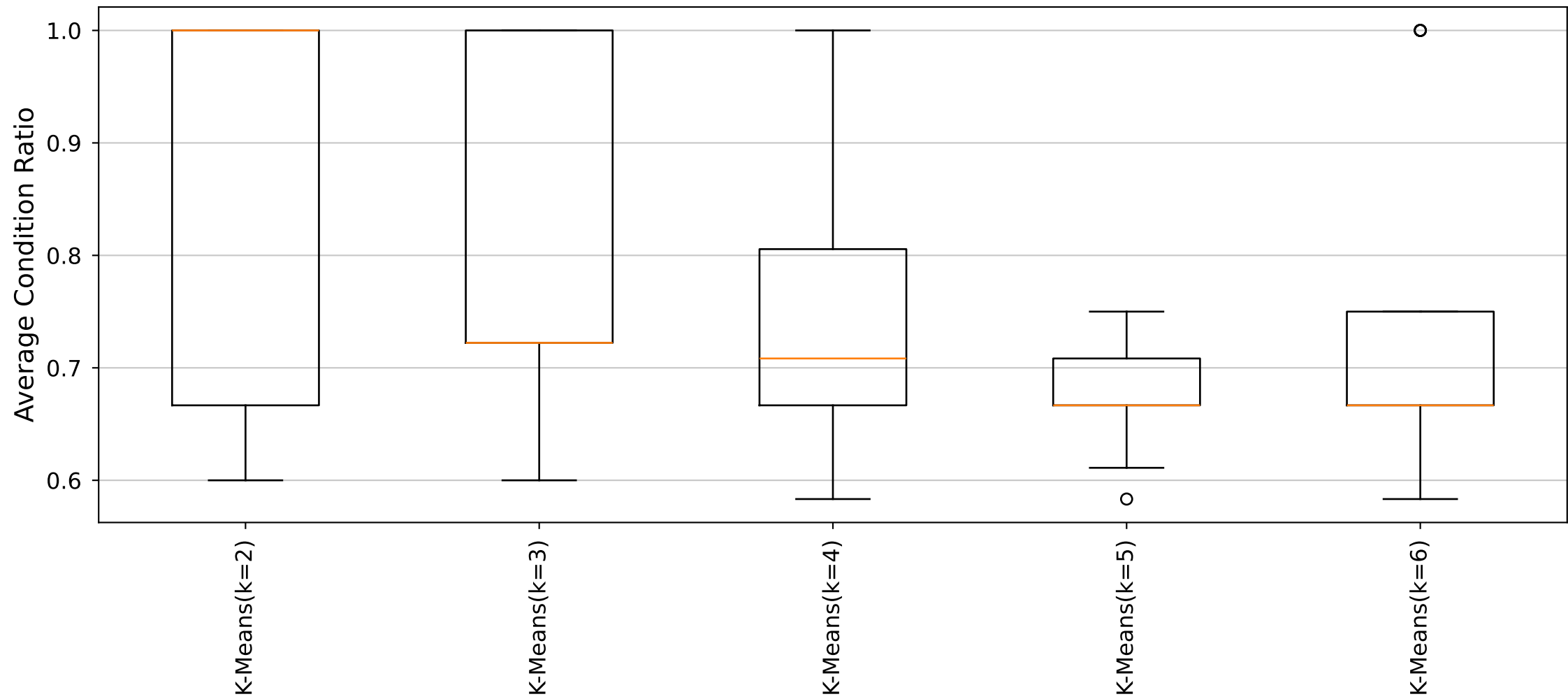
YARA Rules Average Condition Ratio Distribution (Cluster32_Size6 dataset)
